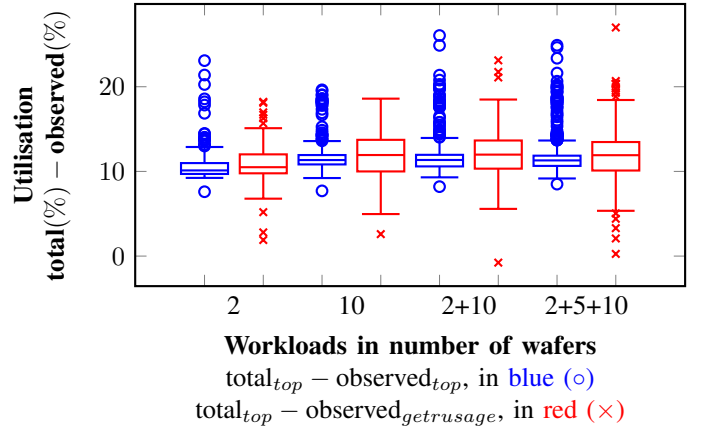
Fig. 5. Behavioural coverage at different stages: CPU utilisation differences for multiple workloads, total system vs. communication-centric view
